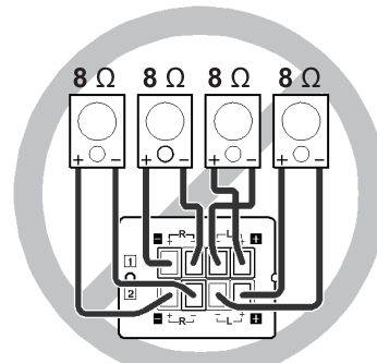
(Speaker terminals)
